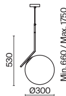
(1) FR5130PL-01BS
